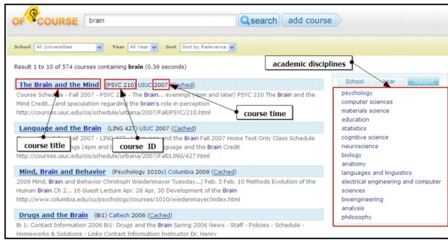
Figure 1: The snapshot of OfCourse of the target pages by crawling only 30% of the entire Web site.
